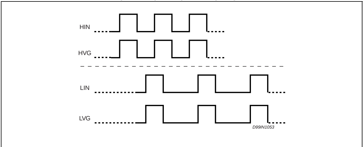
Figure 3. Input/output timing diagram
